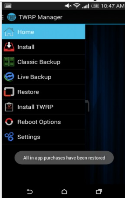
TWRP Manager
