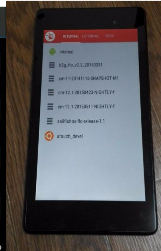
MultiROM Bootloader
