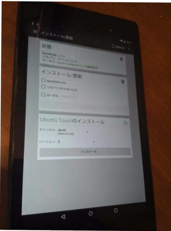
MultiROM Manager
