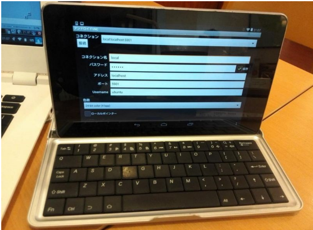
VNC Viewer
