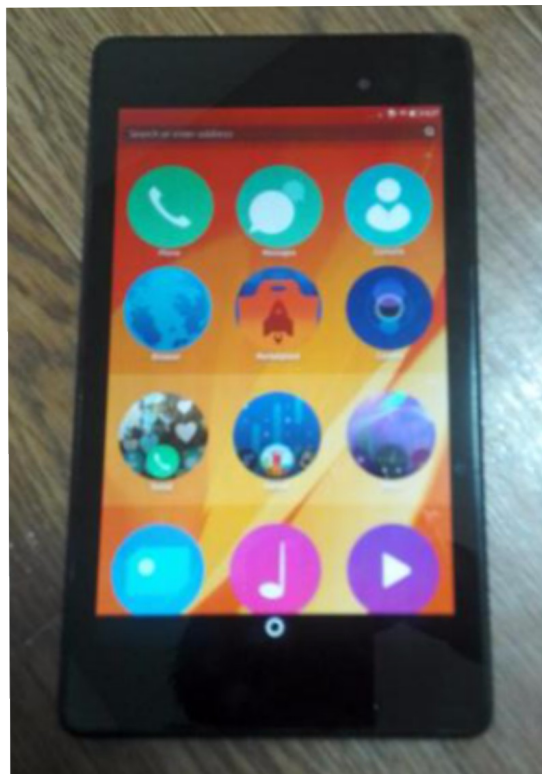
FirefoxOS
