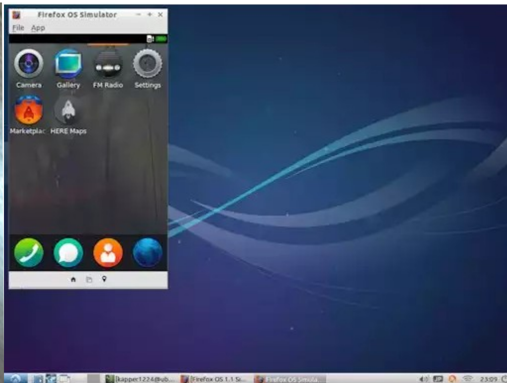
FirefoxOS Simulator
