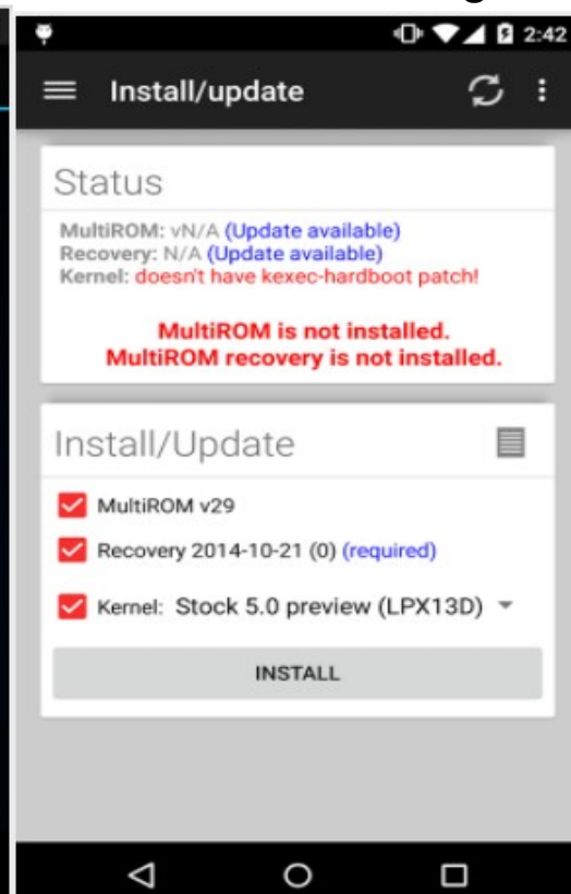
MultiROM Manager
